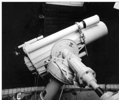
Obr. 5.10: 30-cm astrograf / 1965-2000
