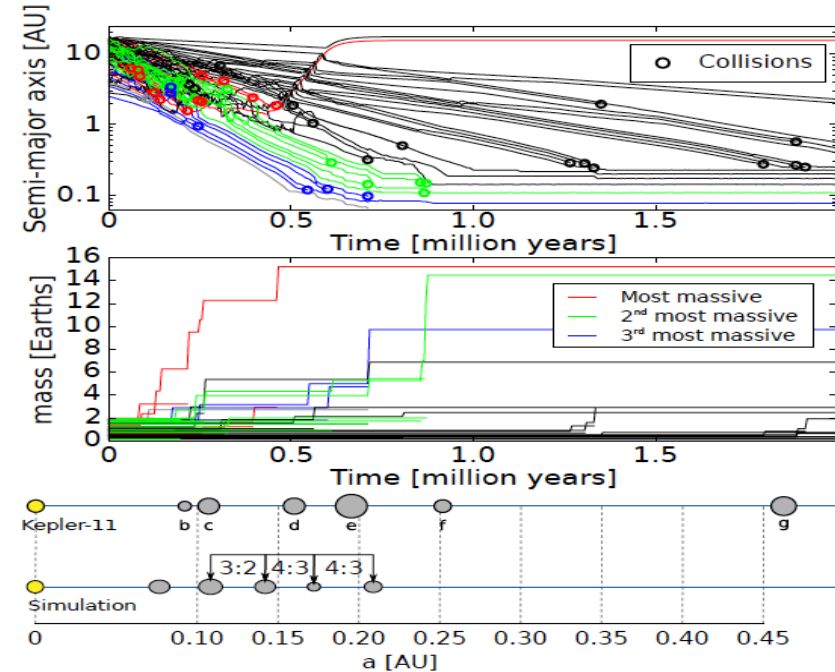
Fig. 6.— Formation of a system of hot Super Earths by type I migration. The top panel shows the evolution of the embryos' orbital radii and the bottom panel shows the mass growth. The red, green and blue curves represent embryos that coagulated into the three most massive planets. All other bodies are in black. Only the most massive (red) planet grew large enough to trigger outward migration before crossing into a zone of pure inward migration. From Cossou et al. (2013) .
