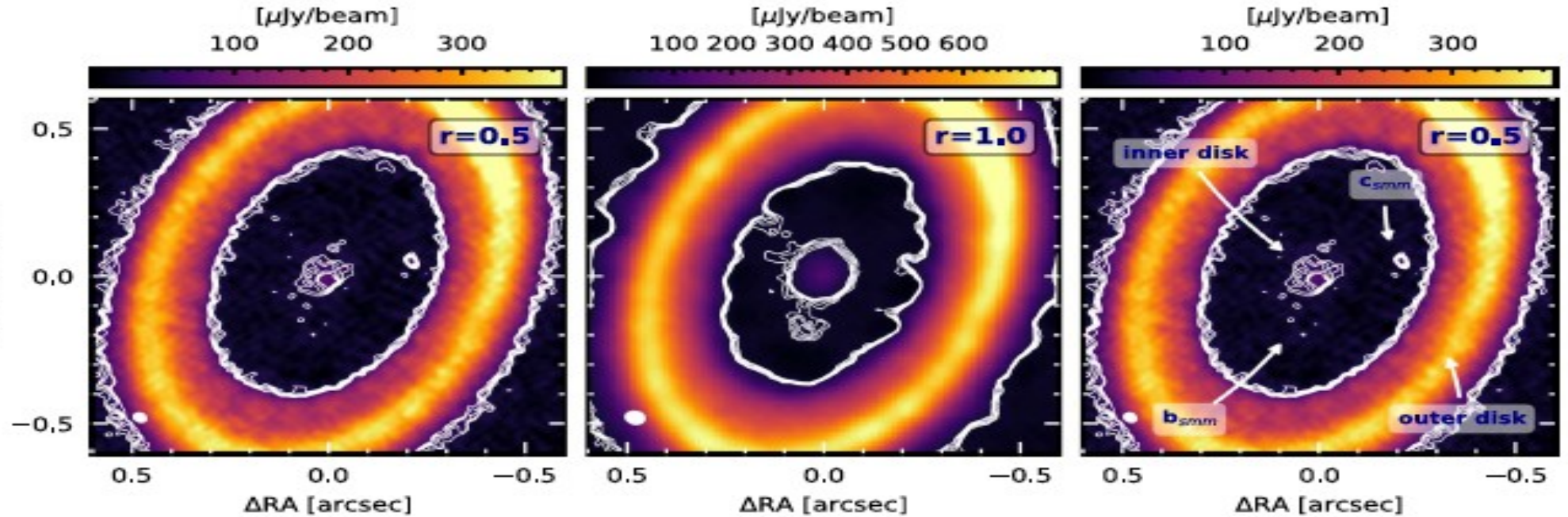
Figure 1. Images of the new continuum observations of PDS 70 (LB19+SB16). The data were imaged with a robust parameter of 0.5 (left panel) and 1 (middle panel), with resolutions of 0''.036 \times 0''.030 and 0''.051 \times 0''.044 , respectively. The right panel shows the same image as in the left panel, with annotations. Beams are in the bottom-left corner of each panel. Contours are 3 to 7\sigma , spaced by 1\sigma (with \sigma = 8.8 and 4.8 \mu\text{Jy beam}^{-1} , respectively). An image gallery for all data sets is given in Appendix A.2.
